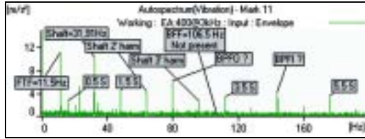
Fig. 8 Envelope spectrum of bearing in lathe
